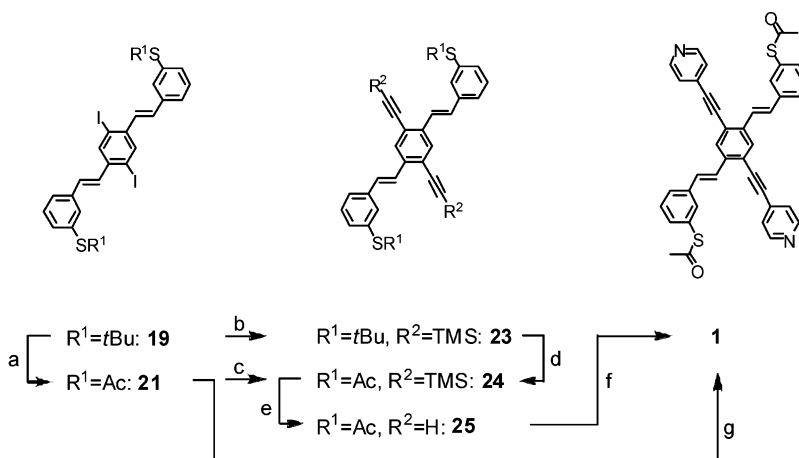
SCHEME 3. Different Strategies for the Assembly of the OPE Subunit of the Cruciform 1 a
