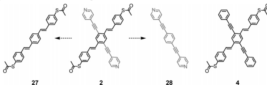
SCHEME 4. The Cruciform 2 and Its Intrinsic Molecular Rod Fragments 27 and 28 , Together with the Cruciform 4 Lacking the Pyridine Nitrogens as Potential Anchor Groups at the End of the OPE Rod
