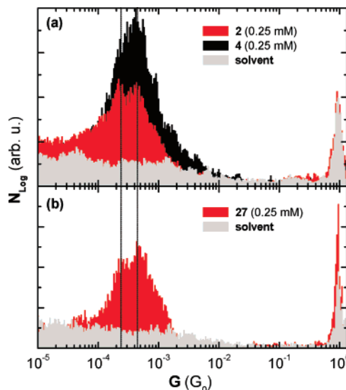
FIGURE 3. (a) Conductance histogram for the pure solvent (gray), 2 (red), and 4 (black). The histograms are made out of 200 consecutive conductance curves. (b) Characterization of OPV ( 27 ) (red) as a reference compound. The histogram is made of 100 consecutive conductance curves. All histograms were normalized to allow a proper comparison. The solvent was a 0.17 mM TBAOH solution in THF/mesitylene (1/4).
