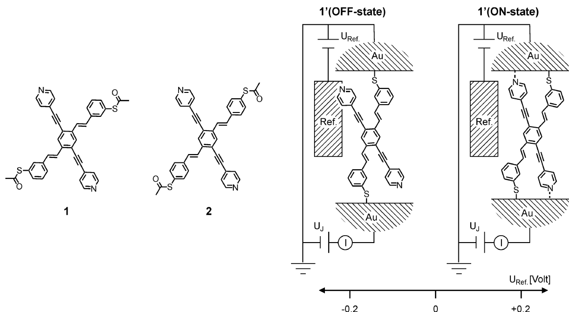
FIGURE 1. Target structures 1 and 2 and hypothesized potential dependent switching mechanism in an electrochemical setup.
