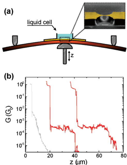
FIGURE 2. (a) Schematics of the MCBJ setup. The sample is inserted in a three-point bending mechanism allowing the controlled elongation of the lithographically patterned Au bridge. Inset: SEM image of the free-standing Au bridge. Scale bar: 500 nm. (b) Typical conductance vs elongation curves for the solvent (gray) and compound 27 (red). Clear conductance plateaus develop when a molecule is trapped within the junction. The solvent was a 0.17 mM TBAOH solution in THF/mesitylene (1/4)
